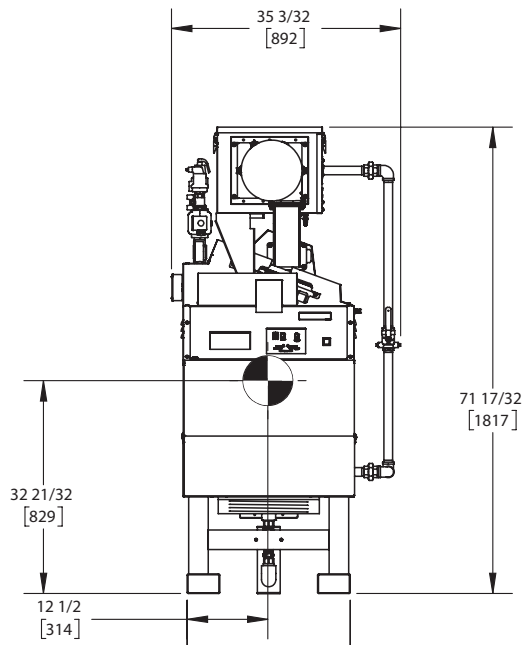
REAR VIEW ASUB-4_L
